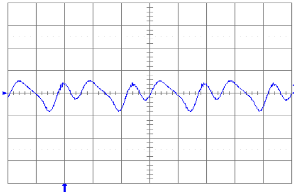
Fig. 1.0V.13: Output voltage ripple (20 mV/div.) at full rated load current into a resistive load with C_o = 10 \mu\text{F} tantalum + 1uF ceramic and V_{in} = 24 \text{ V} . Time scale: 1 \mu\text{s}/\text{div} .
